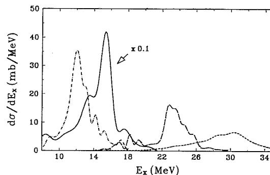
FIG. 3. The cross section for Coulomb excitation of the one-phonon GDR (continuous curve), of the isoscalar GQR (dash-dotted), of the isovector GQR (long dashed), as well as for the double-phonon GDR (short dashed), are shown. They have been calculated at E_{\text{lab}} = 681 MeV/n, taking into account the energy reduction of the beam in the target [5]. The one-phonon GDR cross section has been reduced in the figure by a factor 10.
