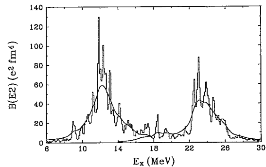
FIG. 2. The transition strength of the giant quadrupole resonance is shown in histogram form. Also shown by the curves are the averaged transition strengths to the left and to the right peaks, corresponding to \tau = 0 and \tau = 1 excitations, respectively.
