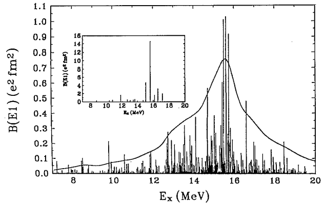
FIG. 1. Fine structure of the giant dipole resonance. The transition strength to each of the microscopically calculated states \Psi_\nu(1\mu) is shown in histogram form. Also shown by the continuous curve is the transition strength obtained introducing an averaging parameter \eta = 500 keV. In the inset, the transition strength obtained in RPA, neglecting the coupling with the two-phonon states, is displayed.
